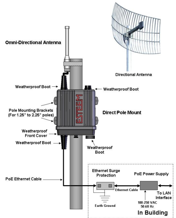
Figure 3. 195Eg Hardware Diagram
