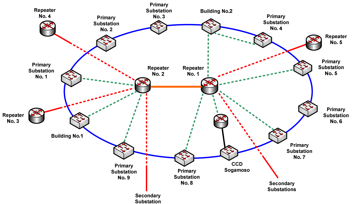
Figure 7. EBSA Network Topology
