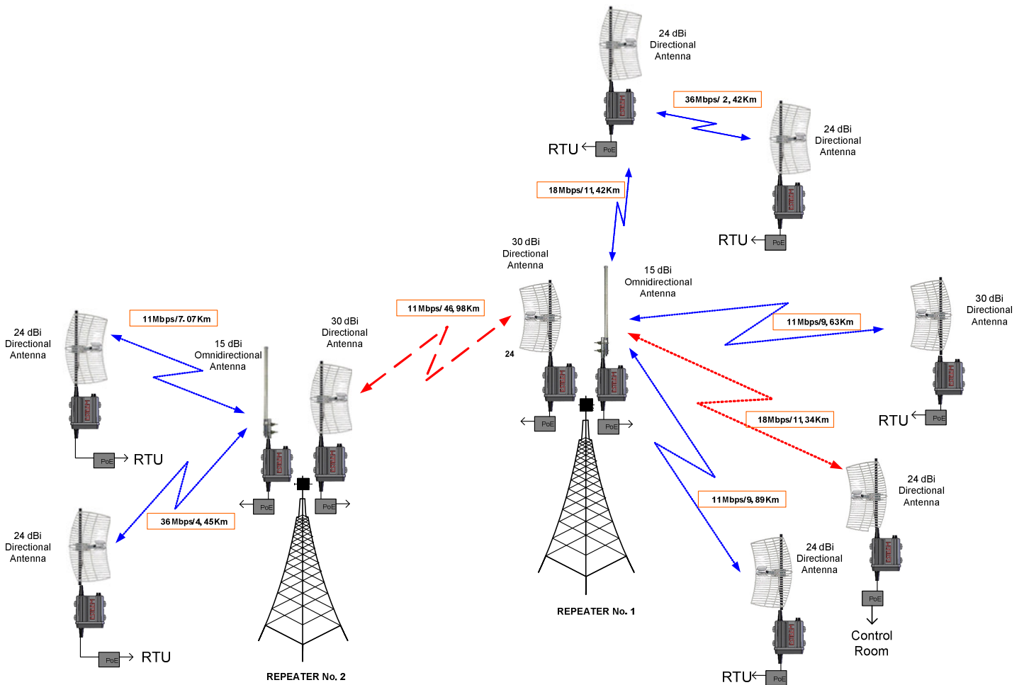
Figure 5. Wireless Network Layout
